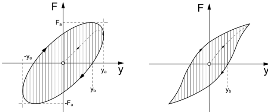
Figure 1. Hysteresis loop a) linear damping b) non linear damping.
