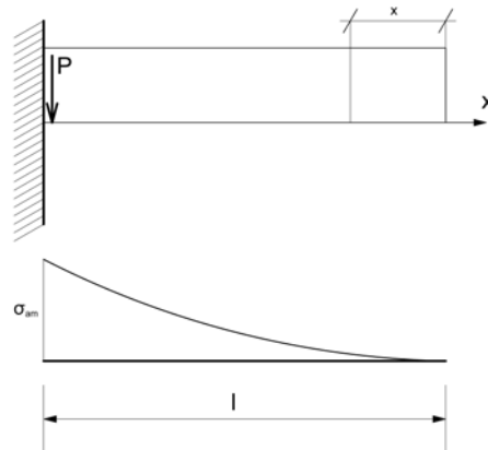
Figure 6. Maximum stress distribution at cantilever beam.
