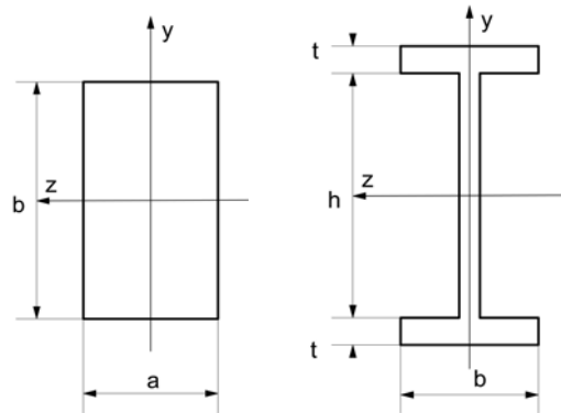
Figure 4. a) rectangular, b) I-section.
