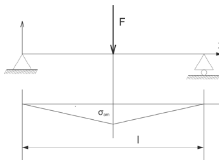
Figure 7. Maximum stress distribution at simply supported beam.
