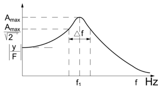
Figure 3. Compliance transfer function for a SDOF system.
