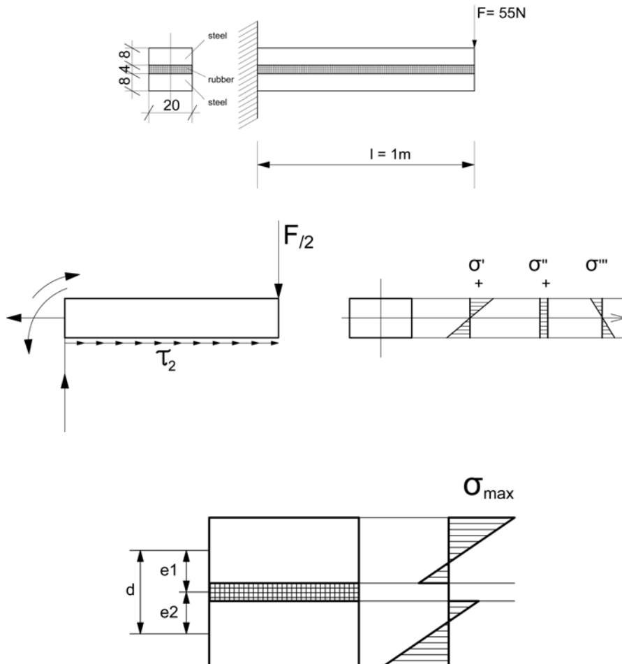
Figure 18. Stress distribution of the sandwich beam.
