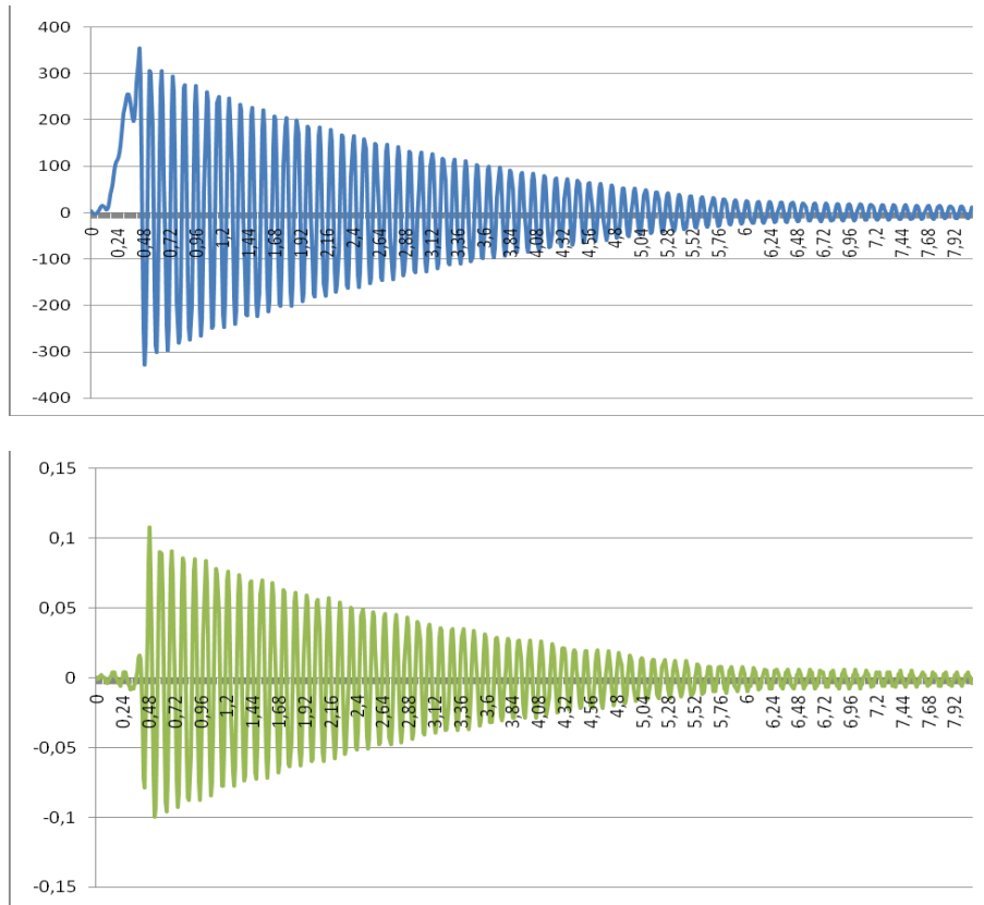
Figure 14. Acceleration of the beam end and strains changing near the fixed point
