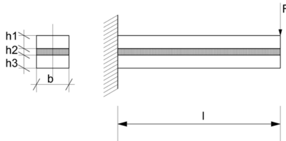
Figure 17. Sandwich beam.
