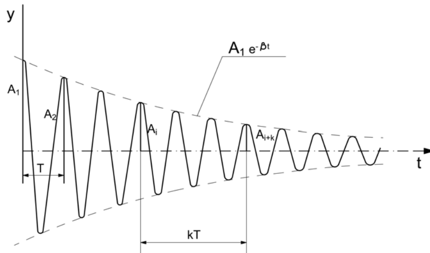
Figure 2. Transient response of a classically under-damped system.
