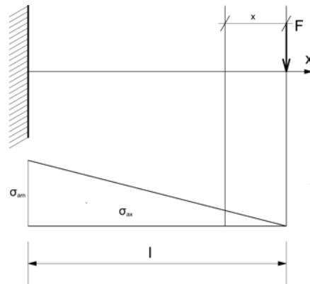
Figure 5. Maximum stress distribution at cantilever beam.
