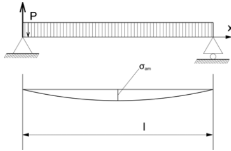
Figure 8. Maximum stress distribution at simply supported beam.
