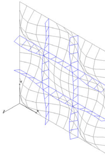
Figure 19. The first vibration mode shape at stiffened plates.
