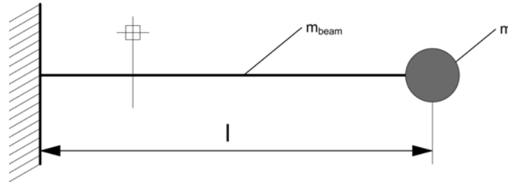
Figure 15. The model of the experiment.
