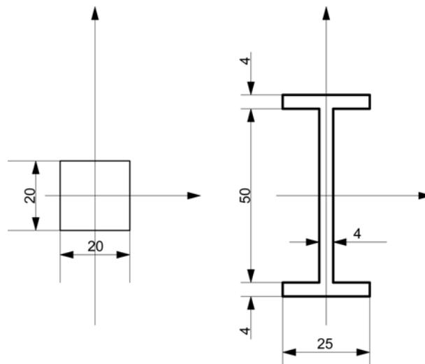
Figure 10. Dimensions of the cross-section.
