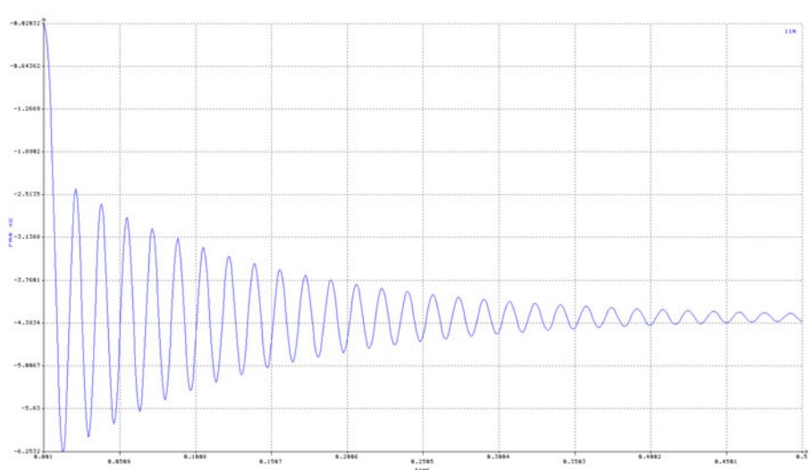
Figure 12. Damped vibration for a fixed beam with an I-section.
