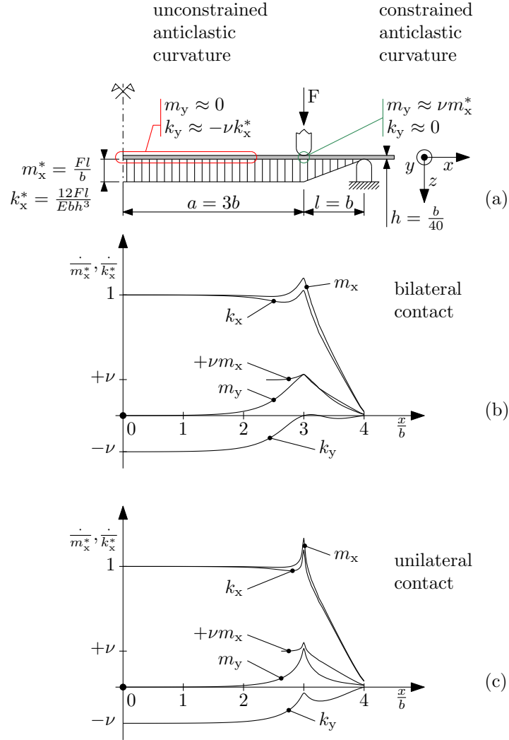
Figure 5: The not-so-trivial four point bending case, where b is the specimen out-of-skip-plane width (we might call it depth ). Moment fluxes and curvatures are sampled at the specimen midwidth, whereas they may vary while moving towards the flanks; the average value of m_x along the width must in fact coincide with m_x^* in correspondence with the load span.
